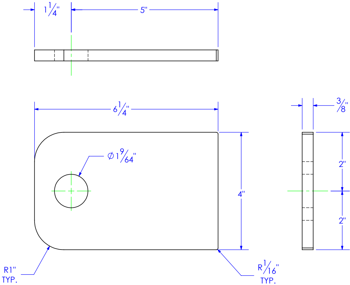
FP-HF3PT-2B PLATE, 3PT MOUNT, LOWER, HF-CARRIER
